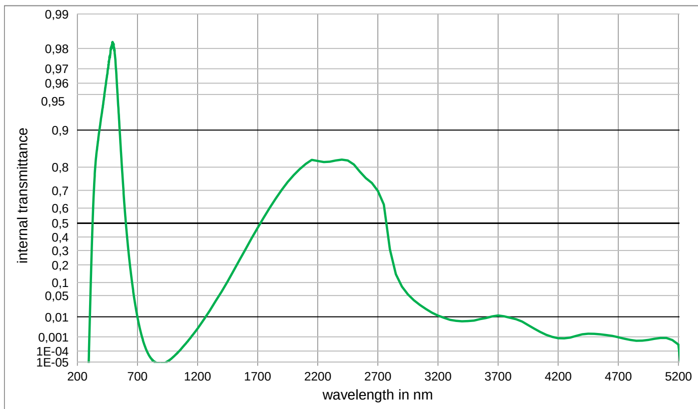
Internal transmittance \tau_i at reference thickness
